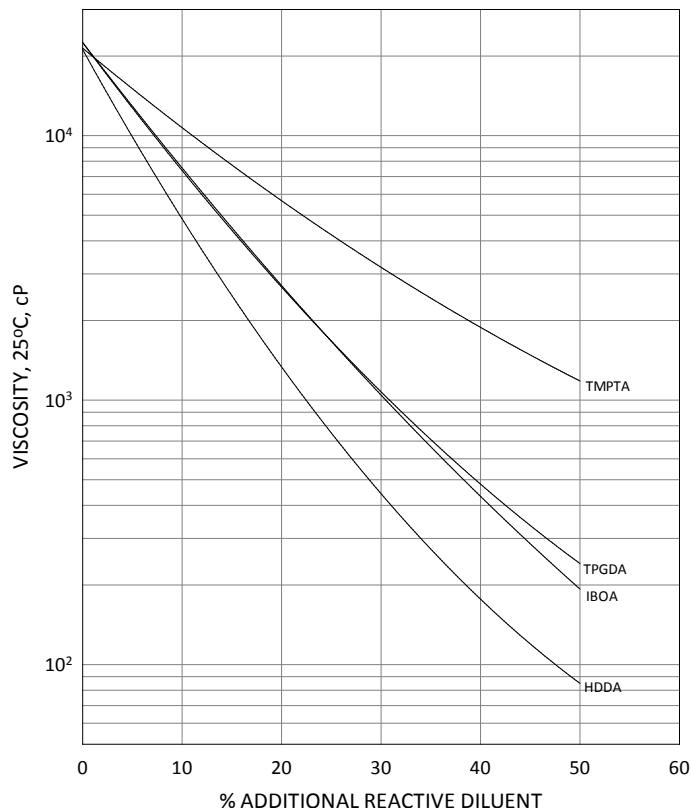
EBECRYL 3730-TP25 - VISCOSITY REDUCTION WITH REACTIVE DILUENTS
