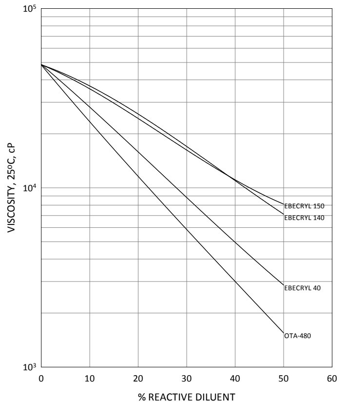
EBECRYL 870 - VISCOSITY REDUCTION WITH REACTIVE DILUENTS
