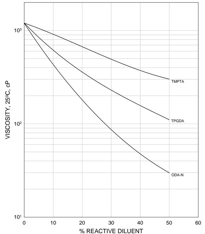
EBECRYL 7100 - VISCOSITY REDUCTION WITH REACTIVE DILUENTS
