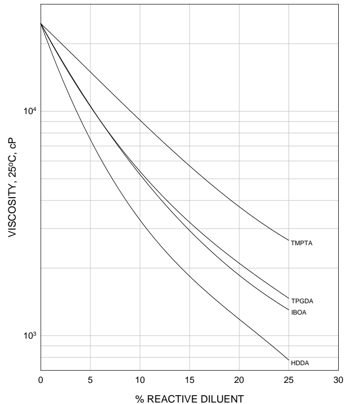
EBECRYL 8301-R - VISCOSITY REDUCTION OF REACTIVE DILUENTS
