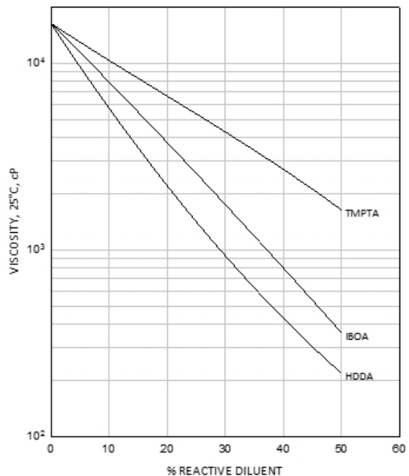
EBECRYL® 8314 - VISCOSITY REDUCTION WITH REACTIVE DILUENTS
