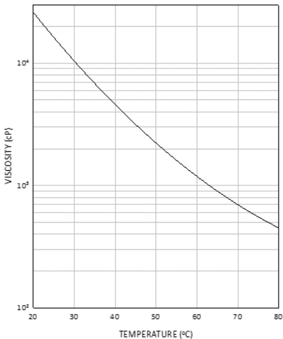
EBECRYL® 8314 - VISCOSITY VS. TEMPERATURE
