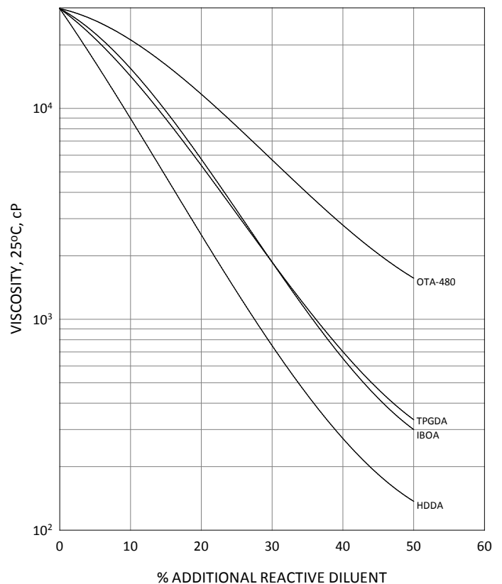
EBECRYL 608 - VISCOSITY REDUCTION WITH REACTIVE DILUENTS
