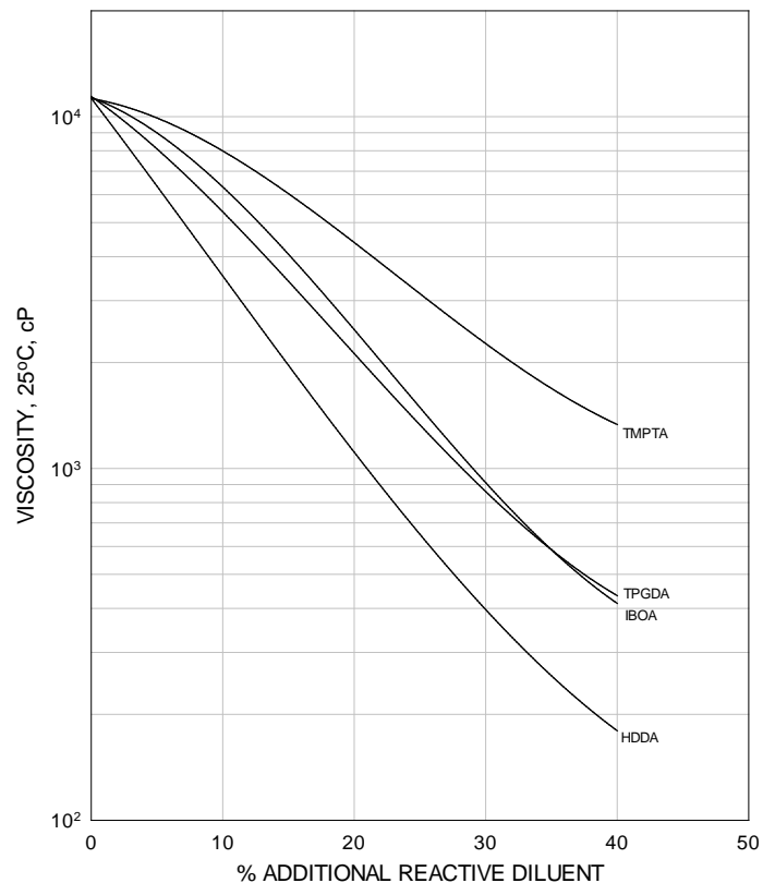
EBECRYL 3720-TP25 - VISCOSITY REDUCTION WITH REACTIVE DILUENTS
