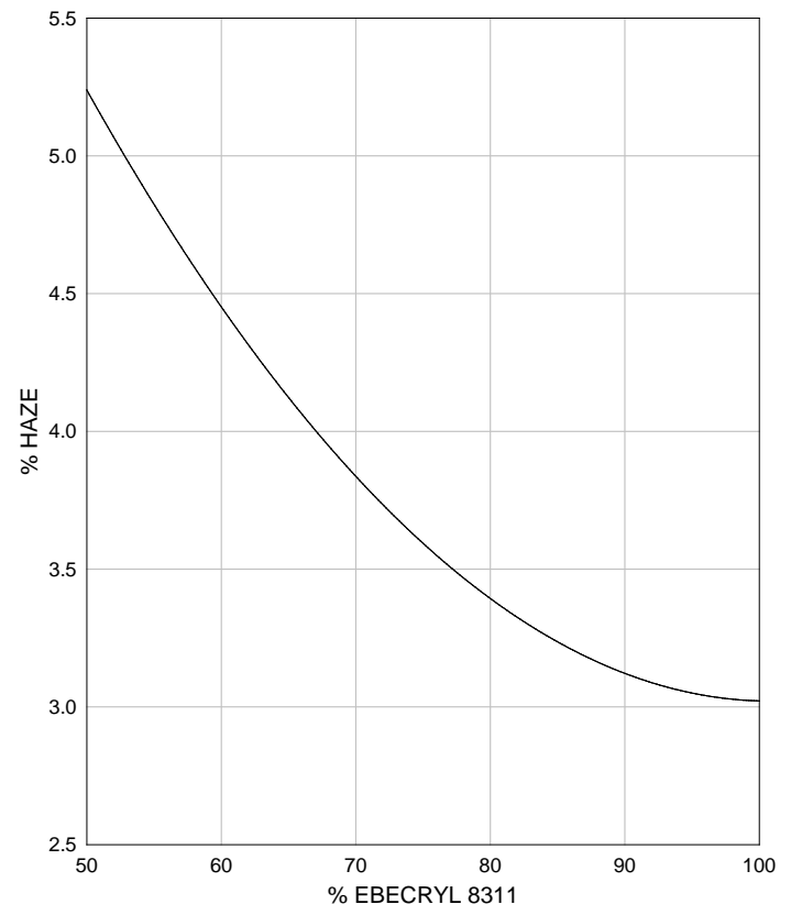
EBECRYL 8311 - HAZE DEVELOPMENT AFTER ABRASION
