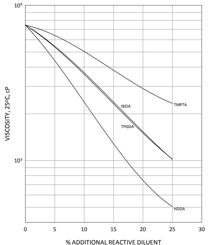
EBECRYL 605 - VISCOSITY REDUCTION WITH REACTIVE DILUENTS
