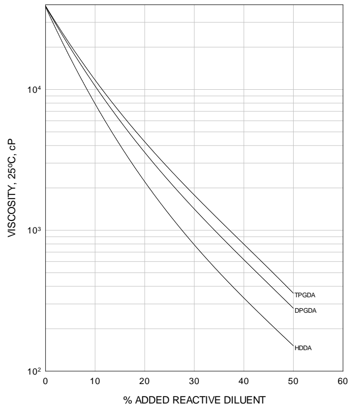
EBECRYL 8501 - VISCOSITY REDUCTION WITH REACTIVE DILUENTS
